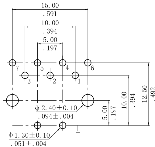
RECOMMENDED HOLE PATTERN
